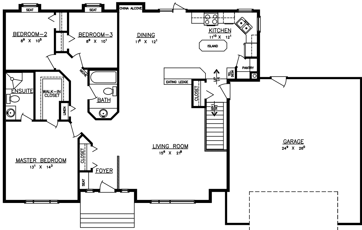
FLOOR PLAN
